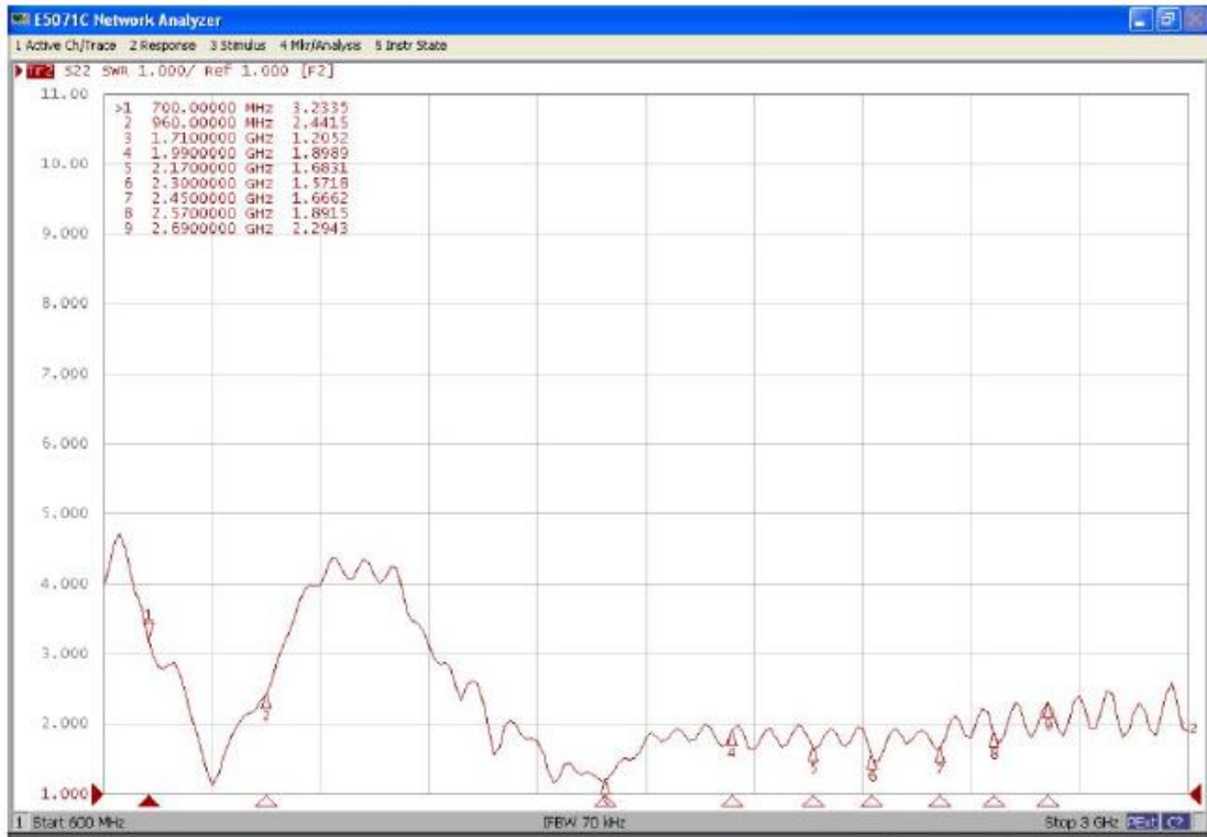
效率及增益(Efficiency And Gain)
